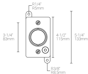
Stainless Steel 316 Flange (S6) EBX-SFD-CSS6
