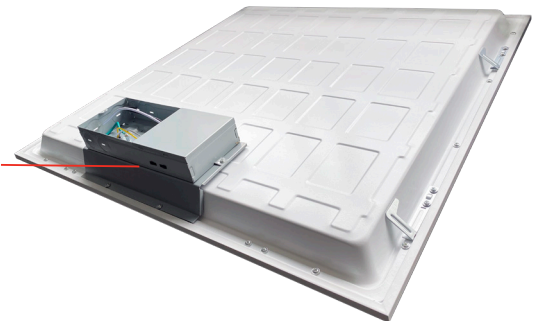
2x2 All-In-One LED Panel (Back View)
