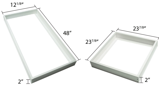
Surface-Mount Kit PLxx-AC-M-V2
