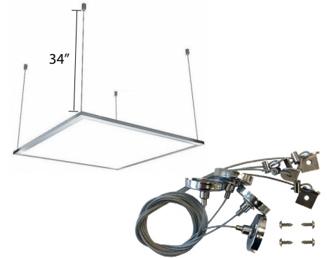
Suspension Kit PL-AC-S
